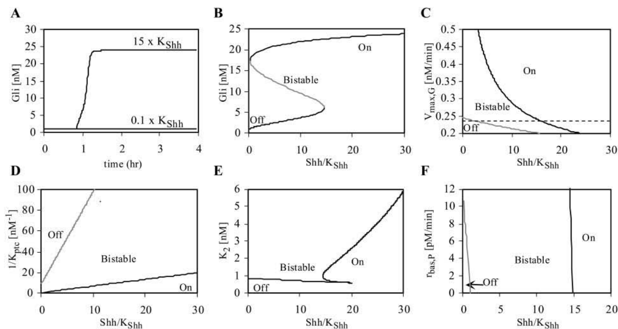
FIGURE 2 (A) Gli trajectories as a function of time at Shh concentrations equal to 0.1 or 15 times its binding constant to Ptc. For the upper curve, the concentration was initially low but was then increased at 0.5 h. (B) Hysteresis in the Shh network, where the network output Gli can attain two possible steady states for an intermediate range of Shh concentration. The point at which switching occurs depends upon whether Shh is increasing or decreasing. (C) Bifurcation, or parameter sensitivity, analysis of how the switching points vary when the gli promoter strength, denoted by v_{\text{max},G} , is changed. A very small change in this parameter has major effects on the Shh levels at which switching occurs. (D) Bifurcation analysis of how the switching points vary with 1/K_{\text{ptc}} , the potency of Ptc inhibition of Smo. (E) Bifurcation analysis of K_2 , the binding affinity of Gli3 for its DNA site, shows that the system is also highly sensitive to this parameter. (F) By contrast, the system or the values of Shh at which switching occurs are not as sensitive to parameters such as r_{\text{bas},P} , the basal rate of Ptc expression.
