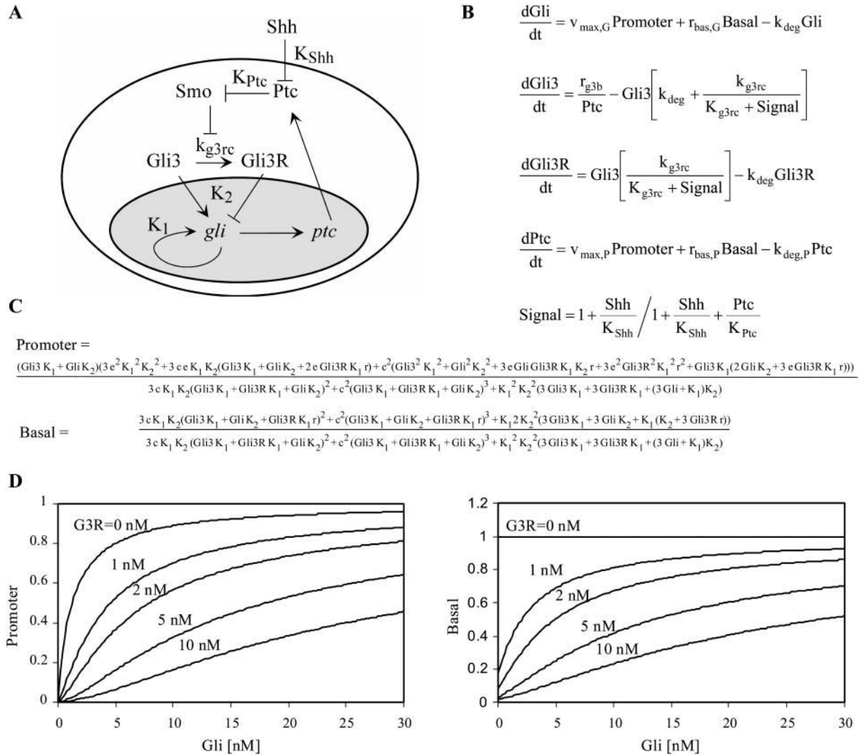
FIGURE 1 (A) Schematic of the Shh signaling system, where Shh binding to its receptor Ptc releases Ptc suppression of the activity of the coreceptor Smo. Smo signaling then inhibits the conversion of the transcription factor Gli3 from an activator to a repressor form. The subsequent accumulation of the Gli3 activator activates the genes gli and ptc . Gli1 binds to and transcriptionally activates its own promoter, as well as that of the signal repressor Ptc. (B) Differential equations that describe the rate of change of the network components depicted in the schematic. (C) Promoter and Basal functions. (D) These functions, which are ratios of polynomials, vary between 0 and 1 and describe how the inducible and basal activities of the gli and ptc promoters vary functionally with the concentrations of the three transcription factors that bind them: Gli3, Gli3R, and Gli. The sigmoidal curves of Promoter and Basal are shown as a function of Gli (with Gli3 = 0) at different levels of the repressor Gli3R.
