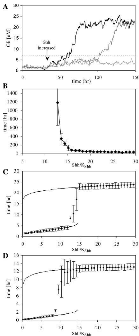
FIGURE 3 (A) Stochastic simulations of Gli trajectories just below the Shh concentration at which the system would deterministically switch from Off to On. When the Gli concentration reaches a threshold value (the unstable, intermediate state in the hysteresis curve of Fig. 2 B, denoted by the dotted line), spontaneous switching occurs. However, one trajectory does not ever switch during the simulation time. (B) The first passage time (FPT) for passage from the Off to the On state as a function of Shh. The mean and standard deviation of 20 simulations are plotted. (C) Stochastic simulations of Gli as a function of Shh. Each point represents the mean and standard deviation of five simulations, each run for 200 h of simulated time. The underlying solid curves are the stable steady states of the deterministic solution from Fig. 2 B. (D) Stochastic simulations of Gli as a function of Shh when Ptc is held constant, eliminating the negative feedback loop. The underlying solid curves are the stable steady states of the corresponding
